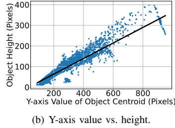
Fig. 8: Y-axis value of object centroid versus object size.
