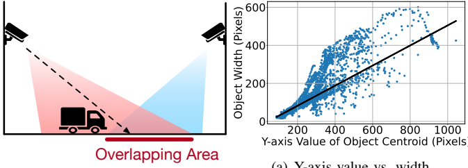
Fig. 7: An illustration of the perspective effect.
