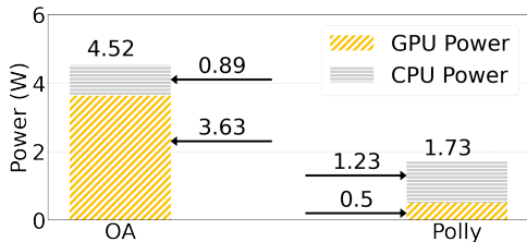
Fig. 16: The average energy consumption comparison between Polly and OA. The object detection model is YOLOv5s.
