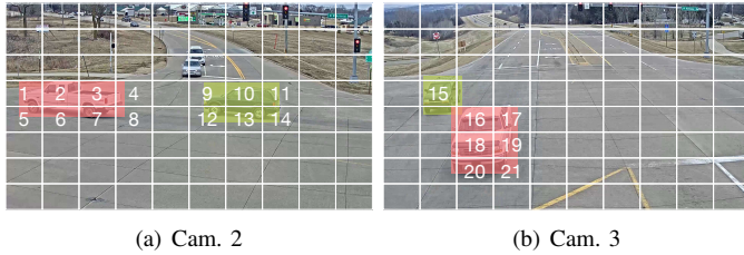
(a) Cam. 2 (b) Cam. 3 Fig. 4: Example of overlap profiling
